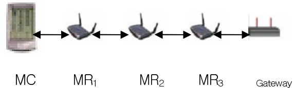
Figure 2: Communication model of mesh network
